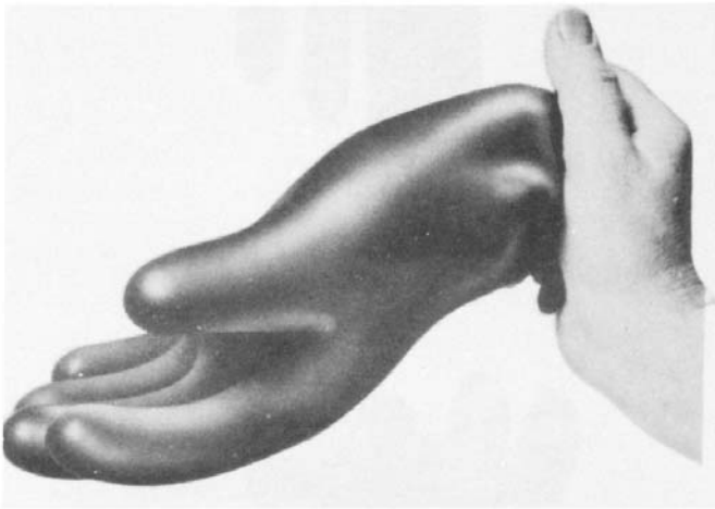
FIG. 45 Inspection
