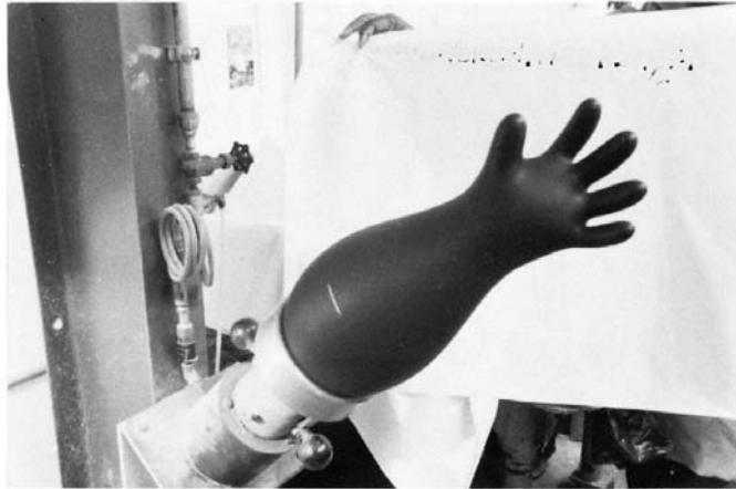
NOTE 1—Glove inflated to maximum allowable degree. FIG. 47 Inflator (Glove Inflated to Maximum Allowable Degree)
