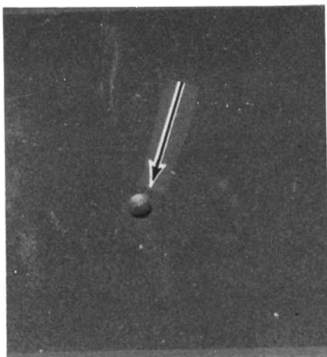
FIG. 22 Pitting
