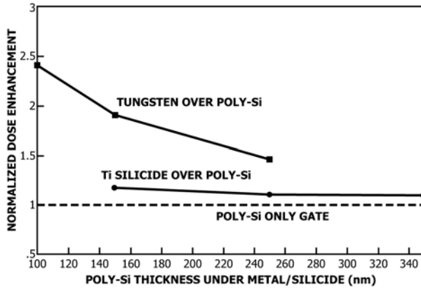
FIG. X1.4 Dose Enhancement Versus Poly-Si Thickness Under the W or \text{TiSi}_2 Layer, Normalized to the Poly-Si-only Case (Benedetto et al (17))
