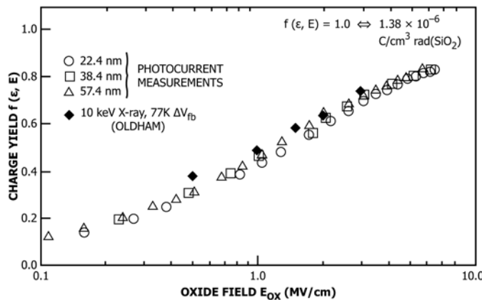
FIG. X1.6 Charge Generation and Fraction of Unrecombined Electron-Hole Pairs Versus Oxide Field
