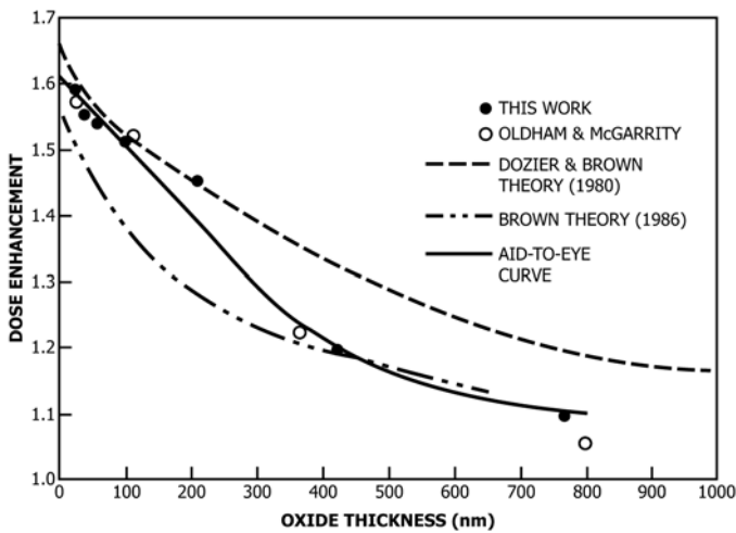
FIG. X1.3 Dose Enhancement Versus Oxide Thickness (From Benedetto and Boesch (10)). Open Circles: Oldham and McGarrity (11). Dashed Line: Dozier and Brown (29)
