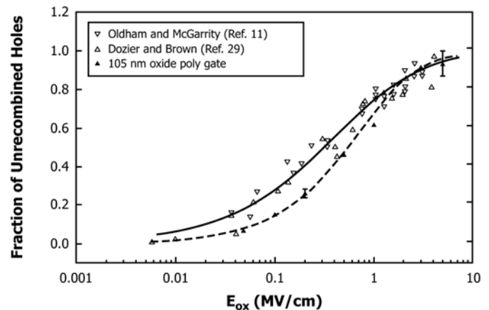
FIG. X1.8 Fraction of Holes That Escape Recombination for Cobalt-60 as a Function of Oxide Field
