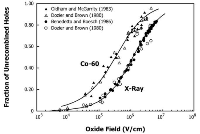
FIG. X1.7 Fraction of Holes Escaping Recombination for Cobalt-60 and 10 keV X-rays as a Function of Oxide Field
