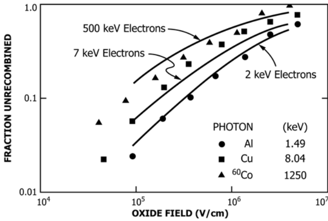
FIG. X1.5 Electron-Hole Pairs Escaping Recombination as a Function of Oxide Field (31)
