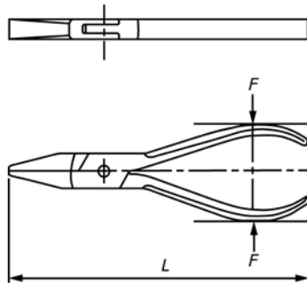
FIG. 21 Insulating Pliers—Bending Test on Legs (see 7.8.2.1)
