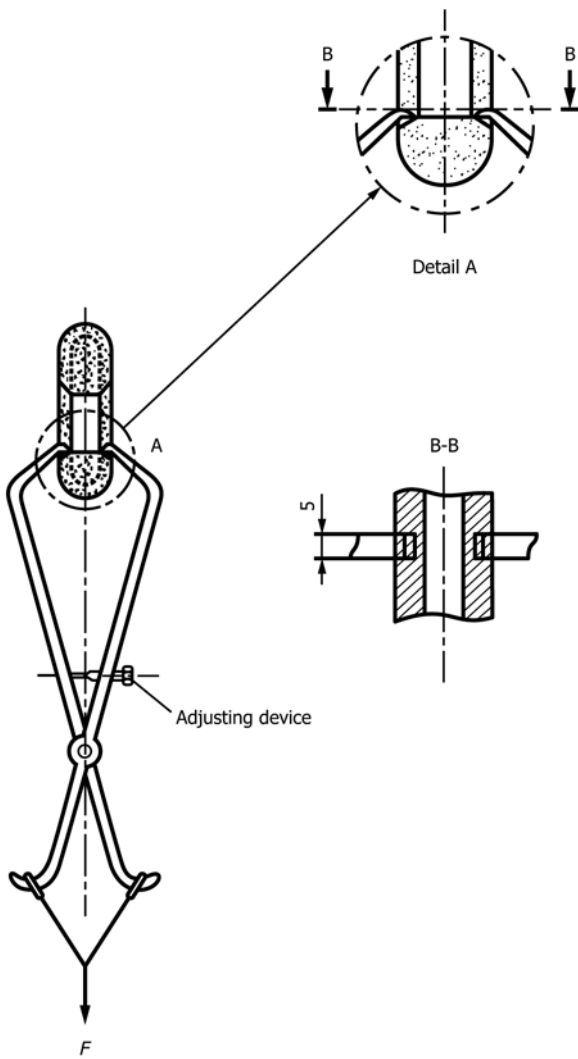
(a) Method B—Test on the Working Head
