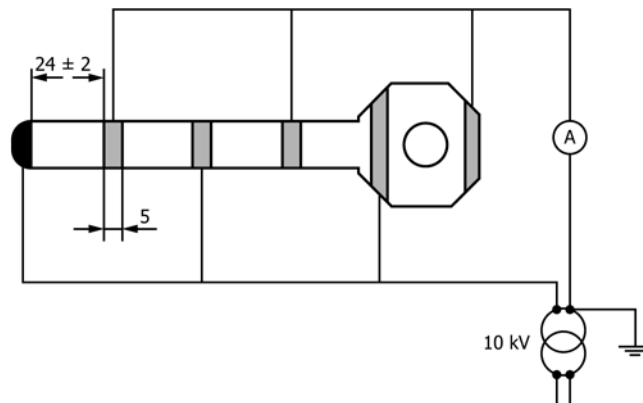
FIG. 14 Dielectric Testing Device for Insulating Tools (see 7.4.4.2)
