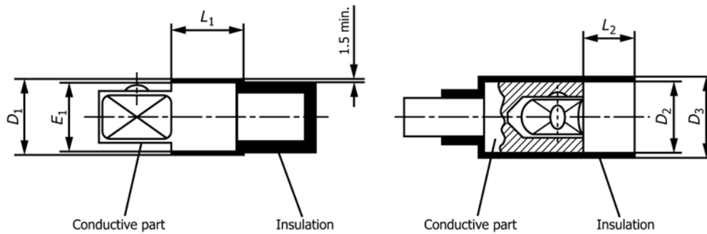
FIG. 13 Description of Dummies for Electrical Tests for Tools Capable of Being Assembled with Square Drives (see 7.4.3.5)
