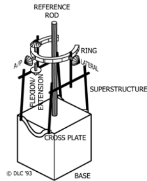
FIG. 3 Attachment of Halo Superstructure
