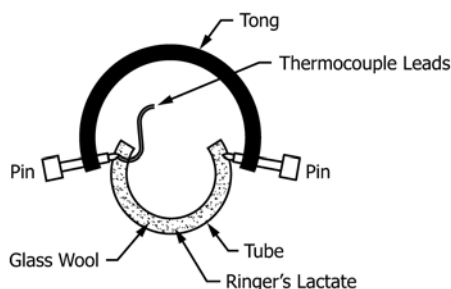
FIG. 5 Model Tong/Tissue System
