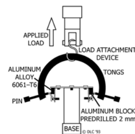
FIG. 1 Suspended Tongs
