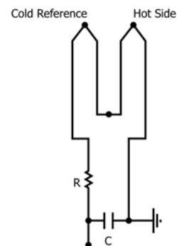
FIG. 6 Circuit
