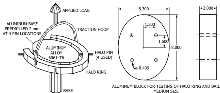
FIG. 2 Suspended Ring
