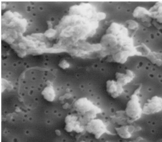
FIG. X2.11 Globular—Agglomerated, Diffuse
