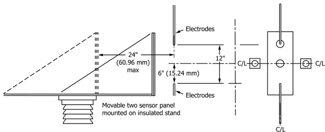
FIG. 3 Sliding Two Sensor Panel
