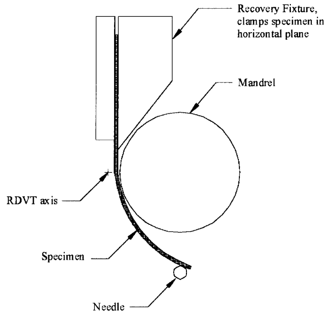
FIG. 4 Placement of Needle on Deformed Specimen, Clamped to the Recovery Fixture. Top View Shown with Stylus and RVDT Removed. Note the Recommended RVDT Axis Location Is Offset from the Mandrel by the Radius of the Needle
