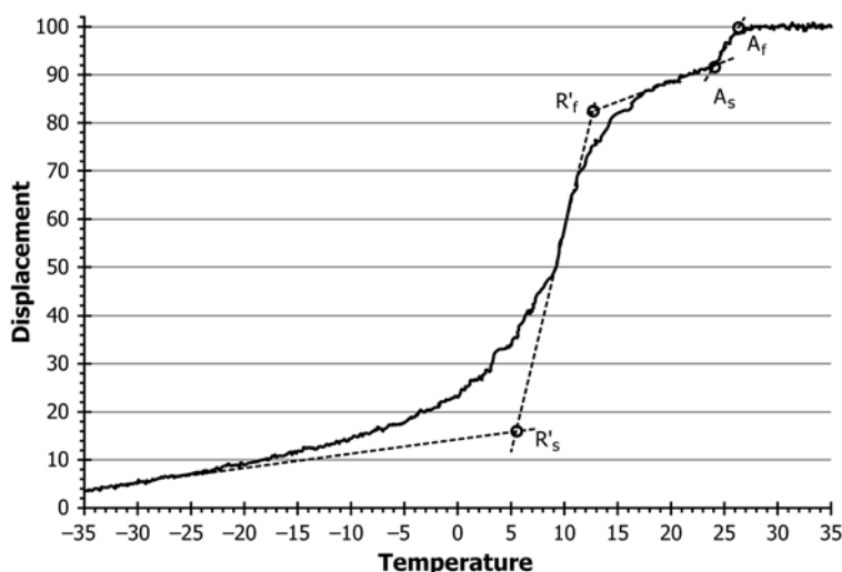
FIG. 6 Two-Stage Transformation—Tangent Lines and Transformation Temperatures
