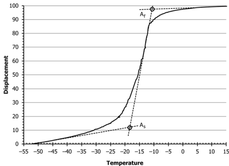
FIG. 5 One-Stage Transformation—Tangent Lines and Transformation Temperatures
