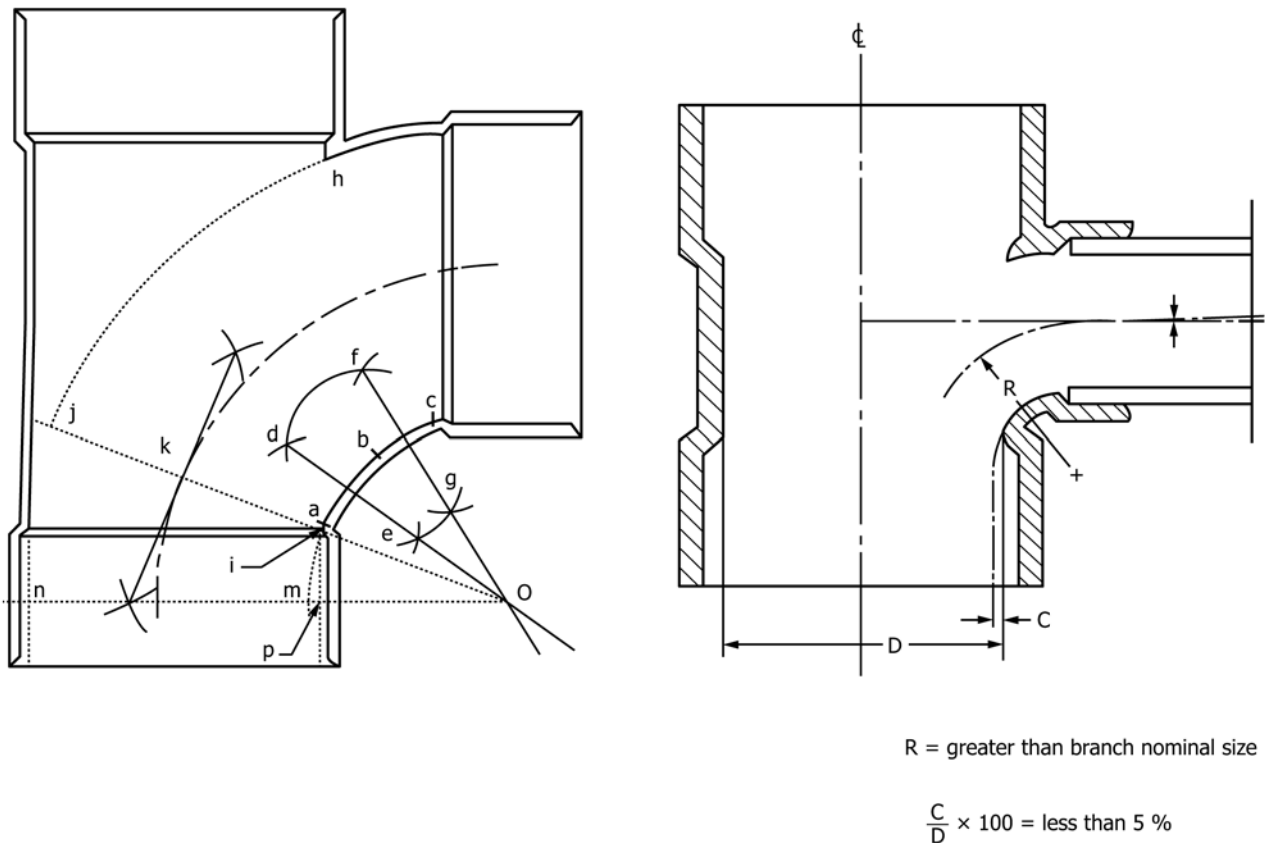
FIG. 1 Measurement for Centerline Radius of Curvature and Branch Alignment
