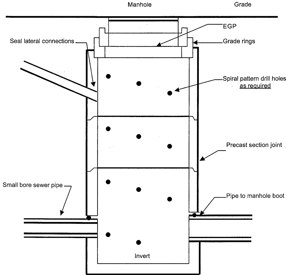
FIG. 1 Manhole with Spiral Pattern Drill Holes
