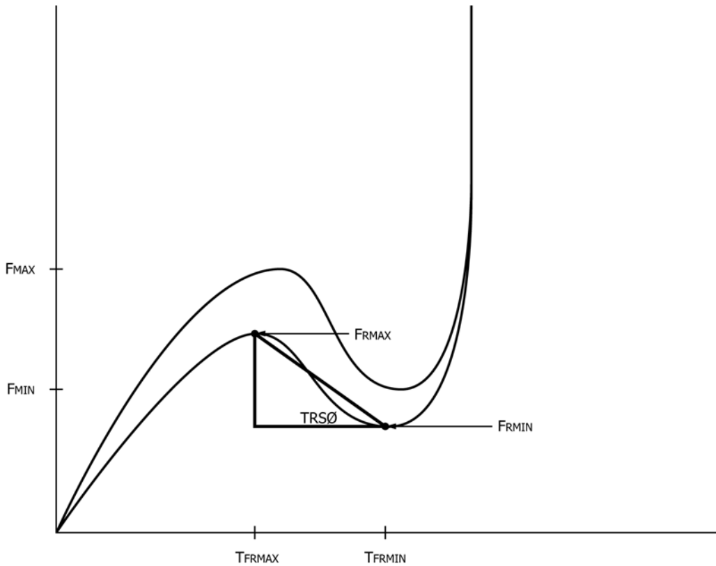
FIG. 4 Tactile Recovery Slope Angle TRSØ
