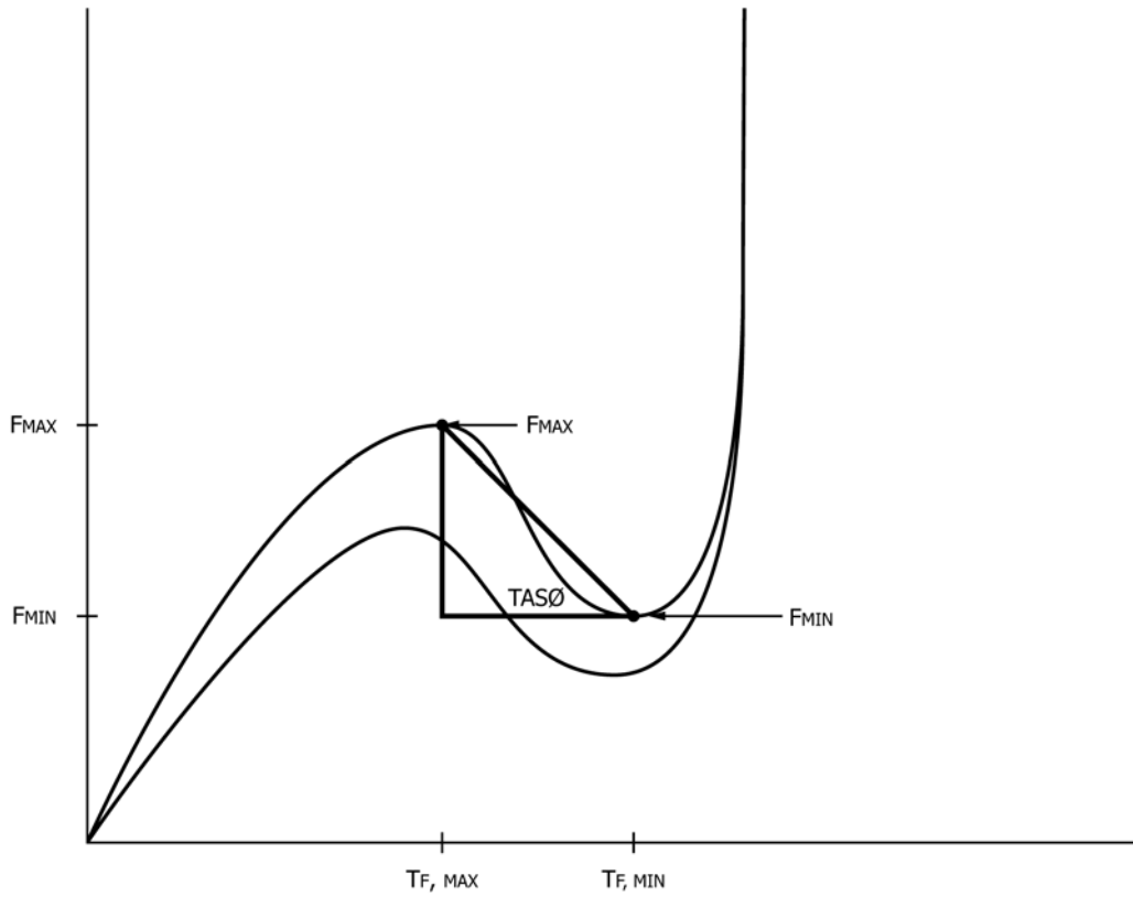
FIG. 3 Tactile Actuation Slope Angle TASØ
