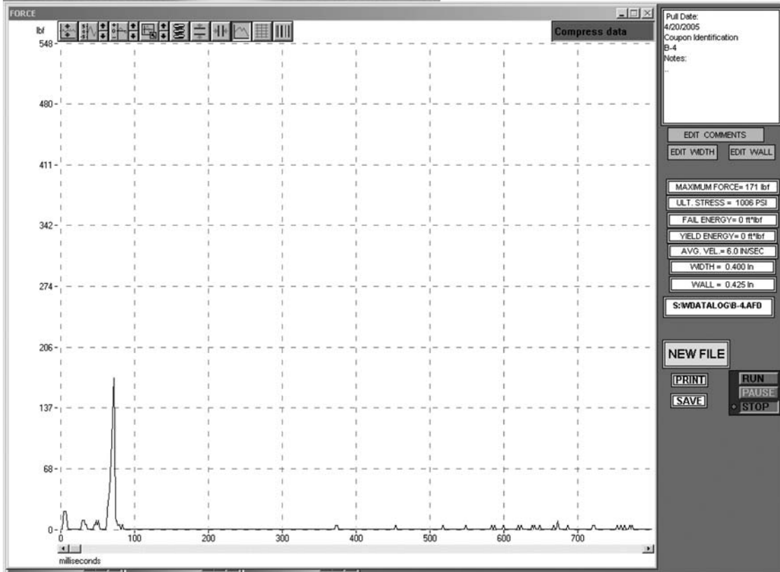
FIG. X1.3 Brittle Rupture
