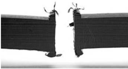
FIG. 1 Brittle Rupture
