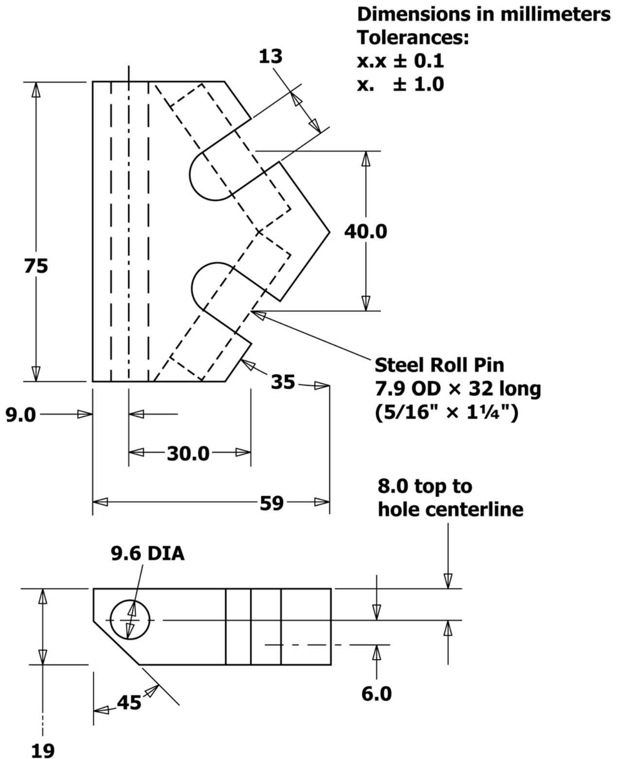
FIG. 7 Cervical Bilateral Polyacetal Block for Hooks, Cables, Wires
