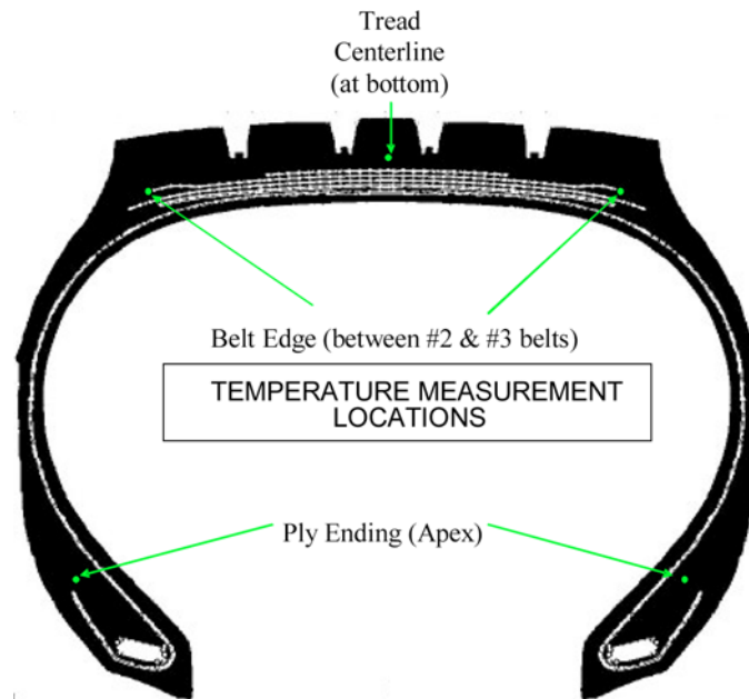
FIG. X1.1 Belt Edge (BE), Centerline (CL), and Ply Ending (Apex) (PE) Temperature Measurement Locations
