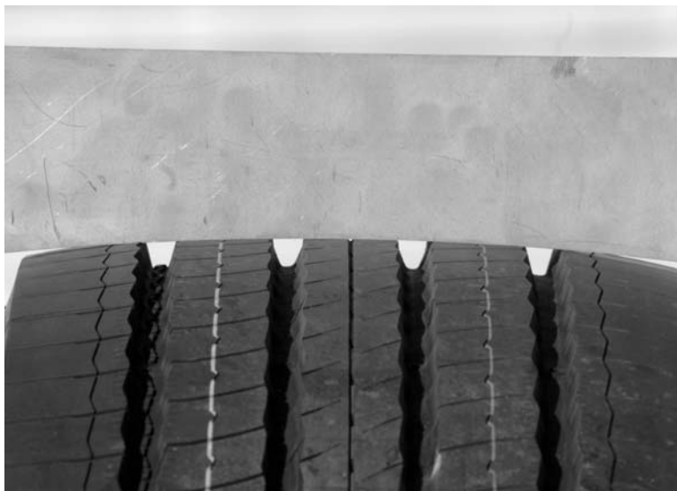
FIG. 4 Measuring a Tread Radius using a Reference Radius Template
