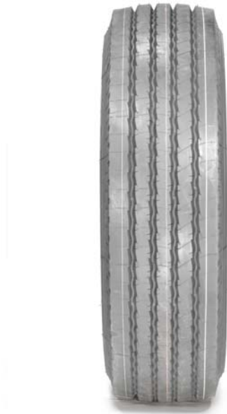
FIG. 1 Front View of the 245/70R19.5 136/134M Radial Truck Standard Reference Test Tire
