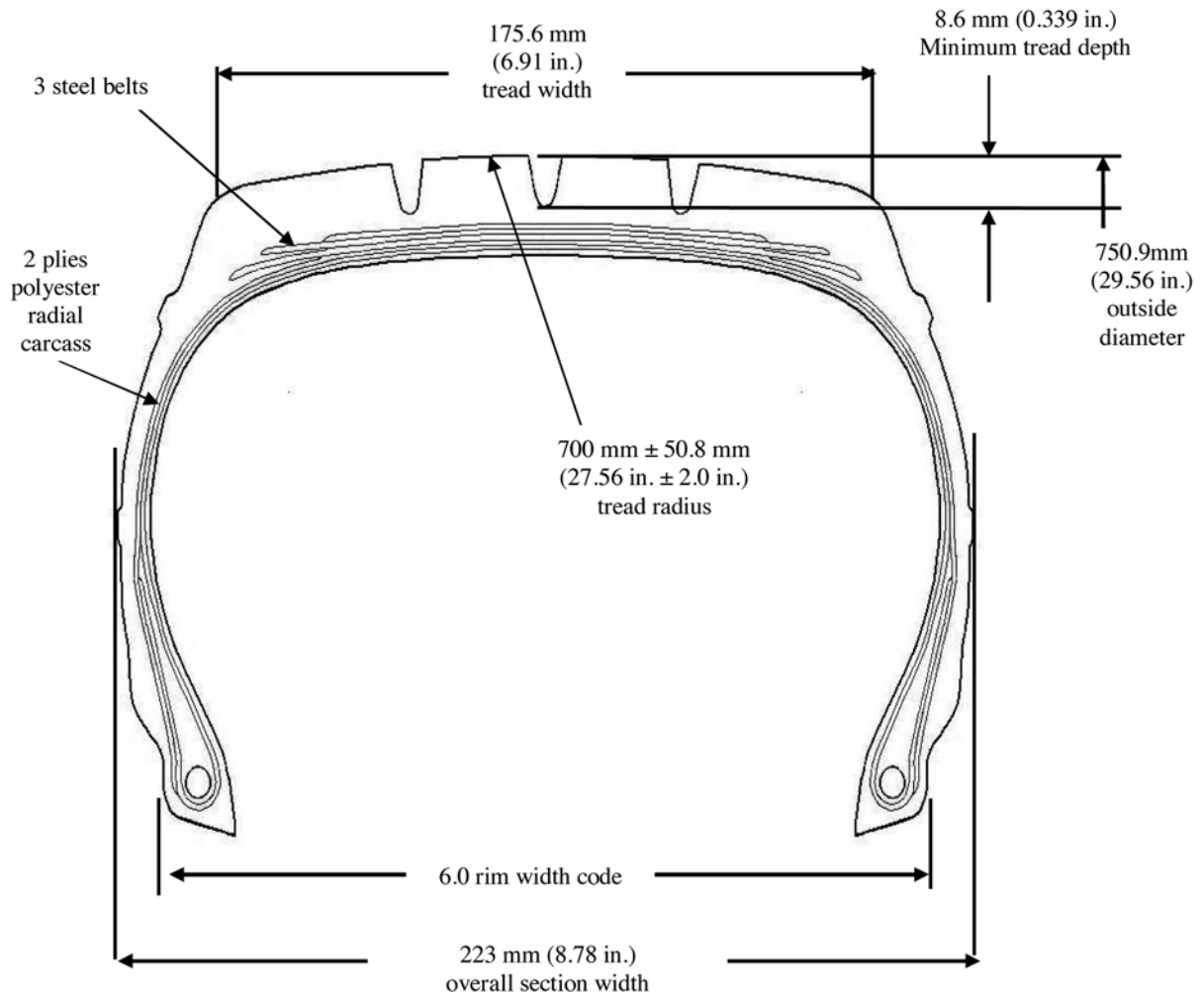
FIG. 3 Tire Cross Section – 225/75R16C 116/114S M+S Radial Light Truck
