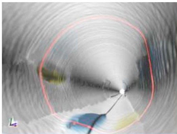
FIG. 2 Still Frame Digital Image of Uneven Deformation of Pipe
