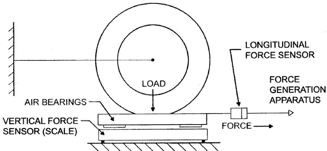
FIG. 3 Force Calibration of Locked Wheel (Alternate Method)
