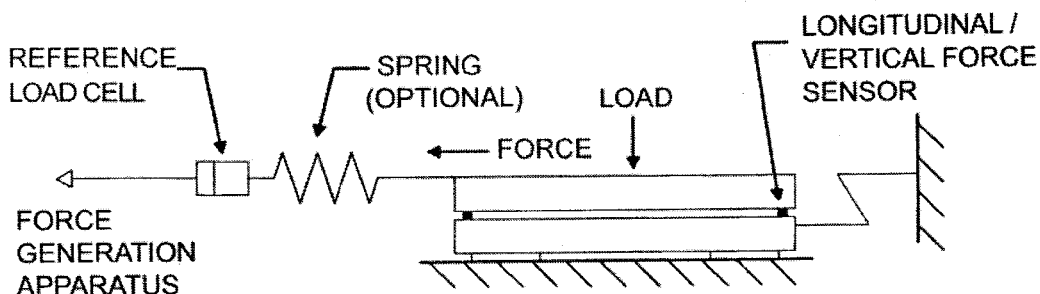
FIG. 1 Force Calibration of a Platform Force Transducer
