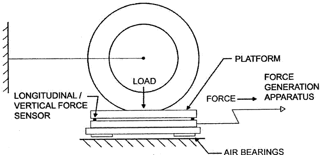
FIG. 2 Force Calibration of a Locked Wheel
