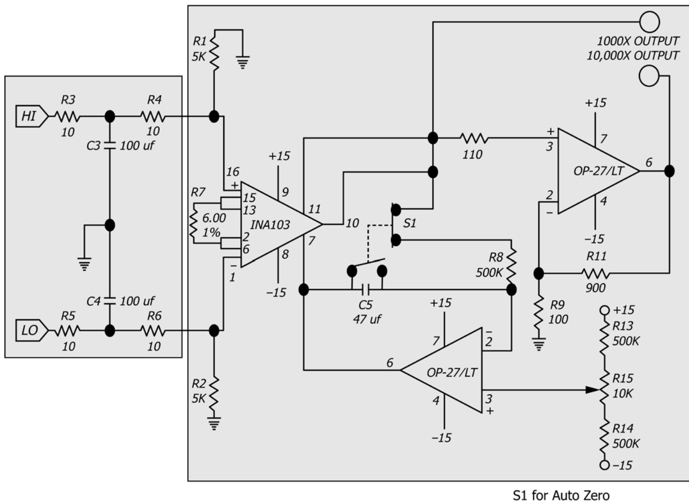
FIG. 2 Recommended Low Noise Amplifier Schematic Diagram
