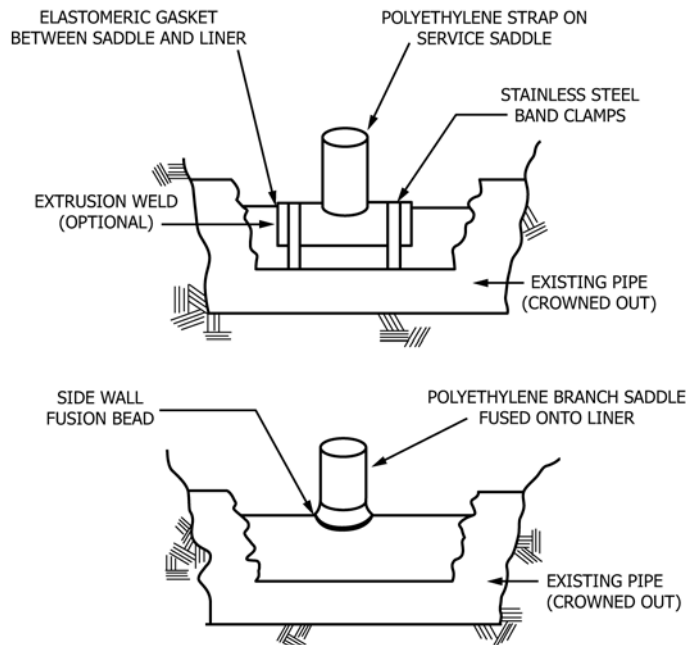
FIG. 8 Lateral Service Connections
