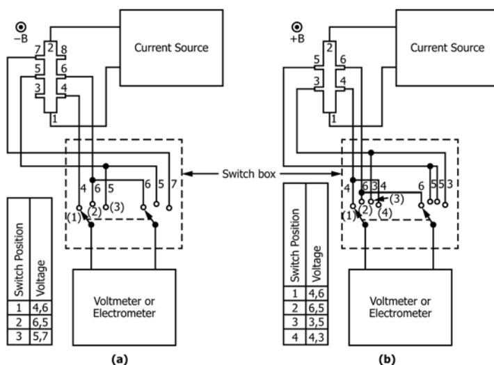
FIG. 6 Representative Test Circuits for Measuring Bridge-Type and Parallelepiped Specimens
