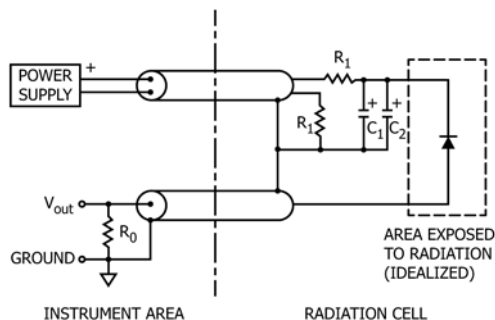
FIG. 2 Typical Irradiation Pulse-Shape Monitor Circuit for Diodes
