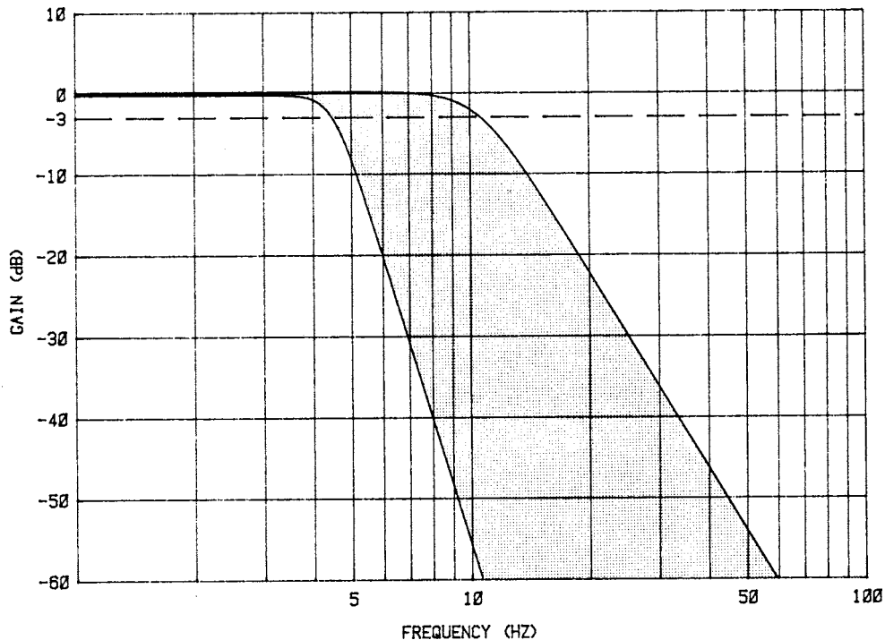
FIG. 2 Filter Frequency Response
