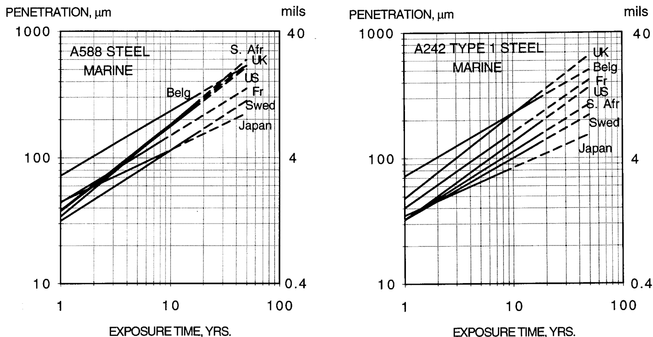
FIG. X1.3 Projected Thickness Loss Per Surface for Specification A588/A588M and A242/A242M Type 1 Steels in Marine Environments in Various Countries
