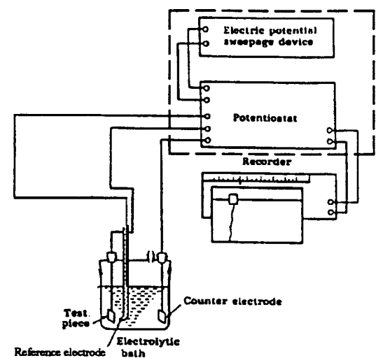
FIG. 3 Schematic Diagram of an EPR Test Apparatus
