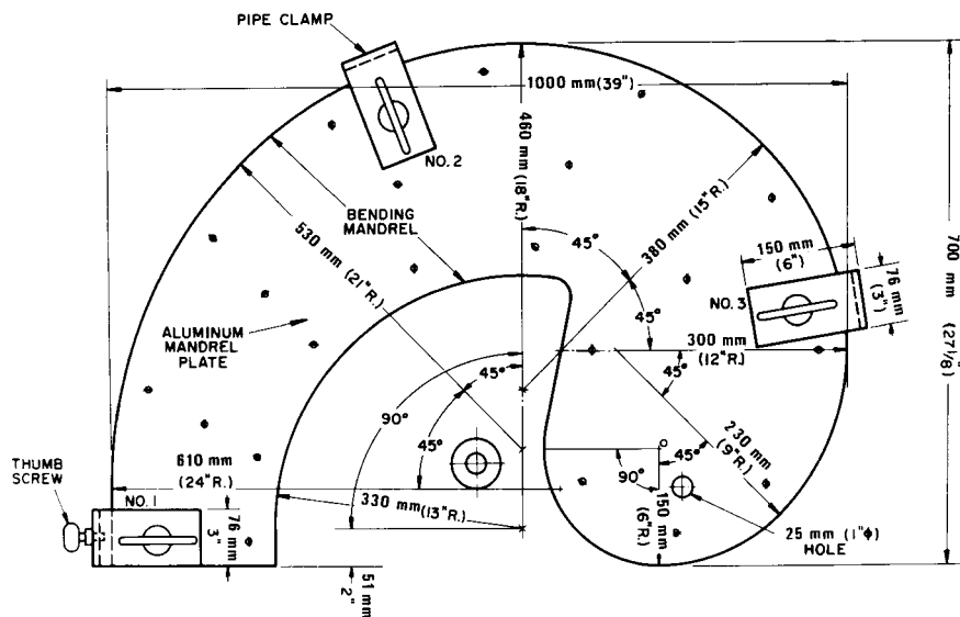
FIG. 1 Variable-Radius Mandrel
