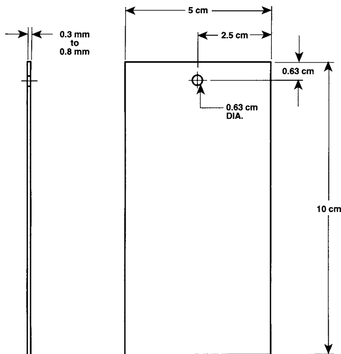
FIG. 1 Standard Test Coupon
