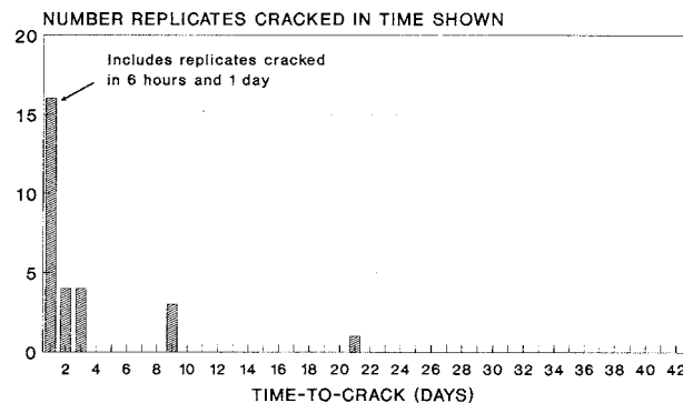
FIG. X1.2 Time-To-Crack for UNS S31600 U-Bends in pH 1.5 NaCl Test
