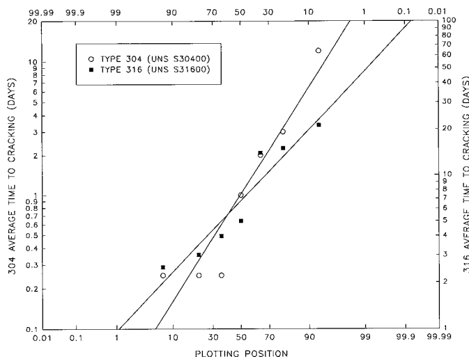
FIG. X1.5 Distribution of Average Cracking Time
