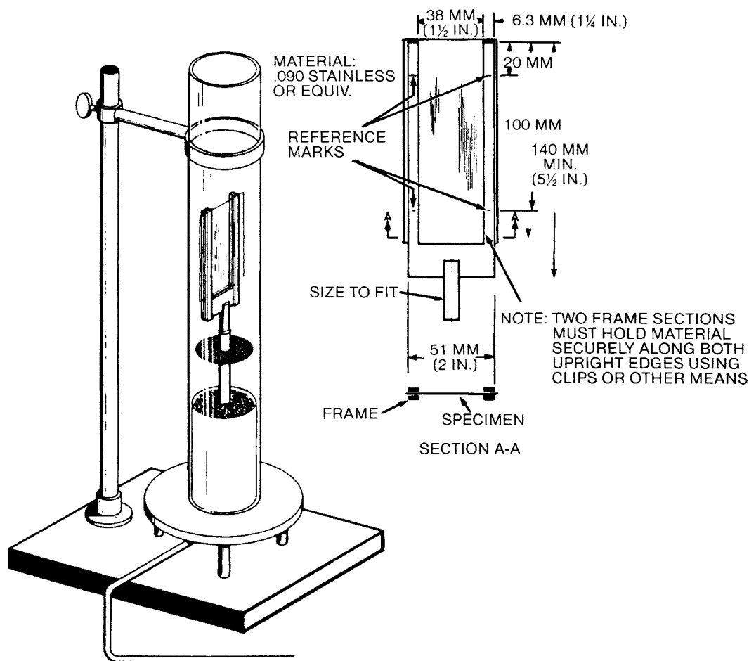
FIG. 2 Frame Design
