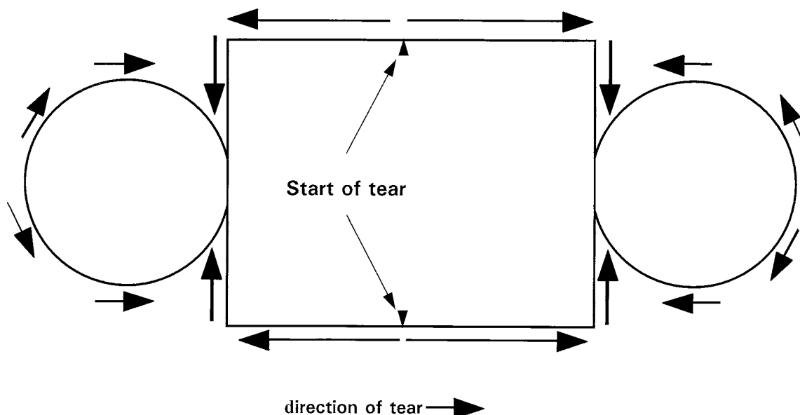
FIG. 1 Illustration of How A Ruptured Cylindrical Vessel Might Look if Fully Flattened
