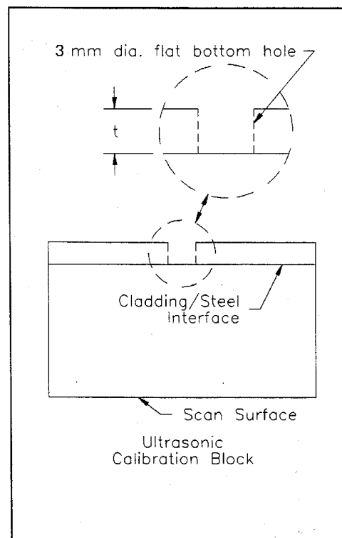
FIG. 4 Ultrasonic Test Calibration Block
