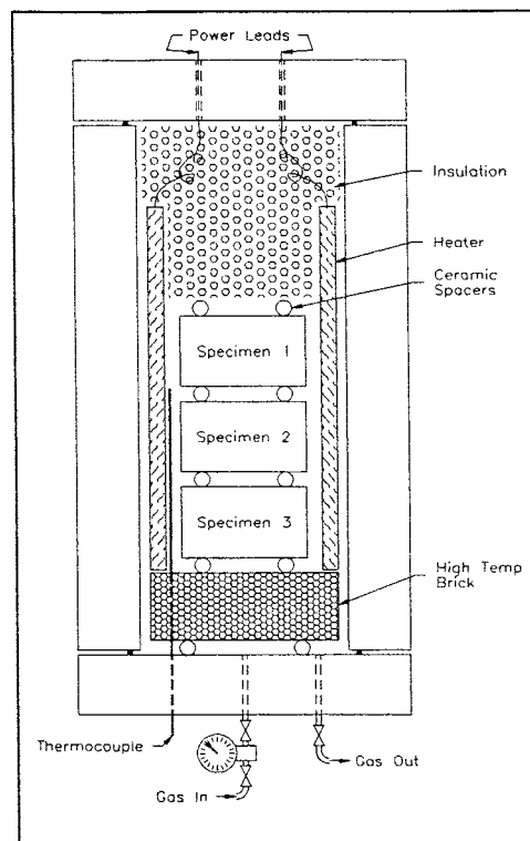
FIG. 2 Typical Test Cell
