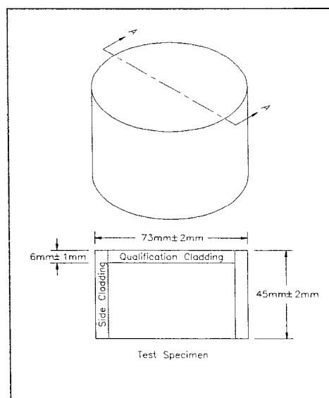
FIG. 3 Test Specimen Configuration
