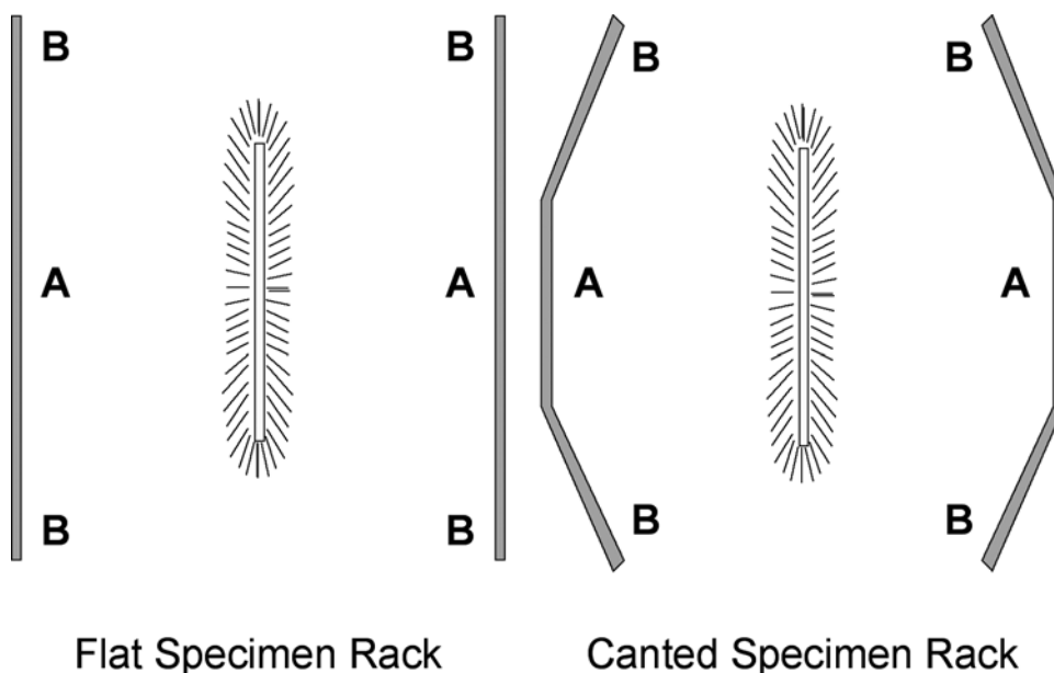
FIG. A1.1 Measurement of Irradiance in Devices Using a Rotating Specimen Rack
