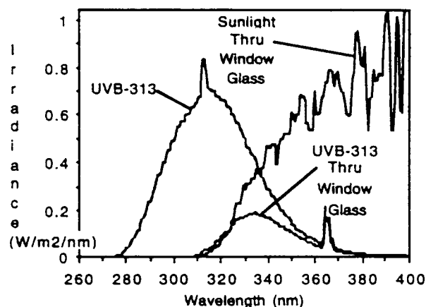
FIG. X1.5 Spectral Power Distributions of Unfiltered UVB-313 Lamp, UVB-313 Thru Window Glass, and Sunlight Through Window Glass
