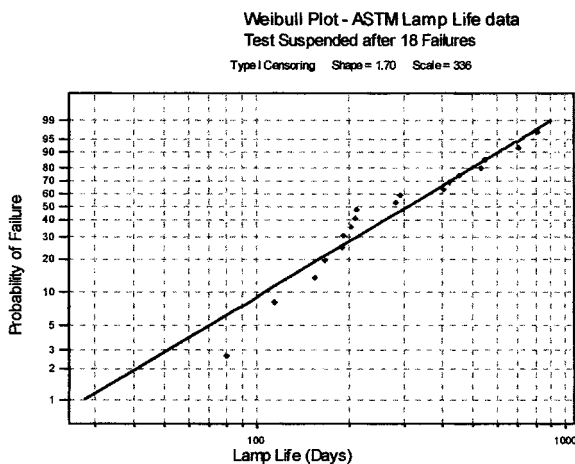
FIG. 4 Percent Probability of Failure Versus Time for Type I Censored Data
