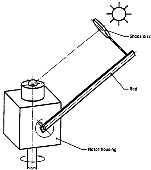
a) Solar tracker with shade disc
