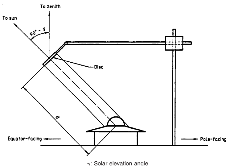
FIG. X1.2 Shade Disc Device Installed Alongside the Pyranometer
