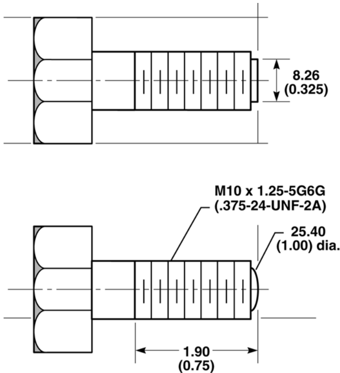
FIG. 4 Bolt Loaded Precracked Double Beam Specimen
