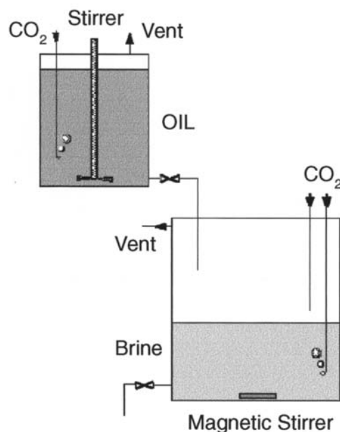
FIG. 14 Partition Vessel
