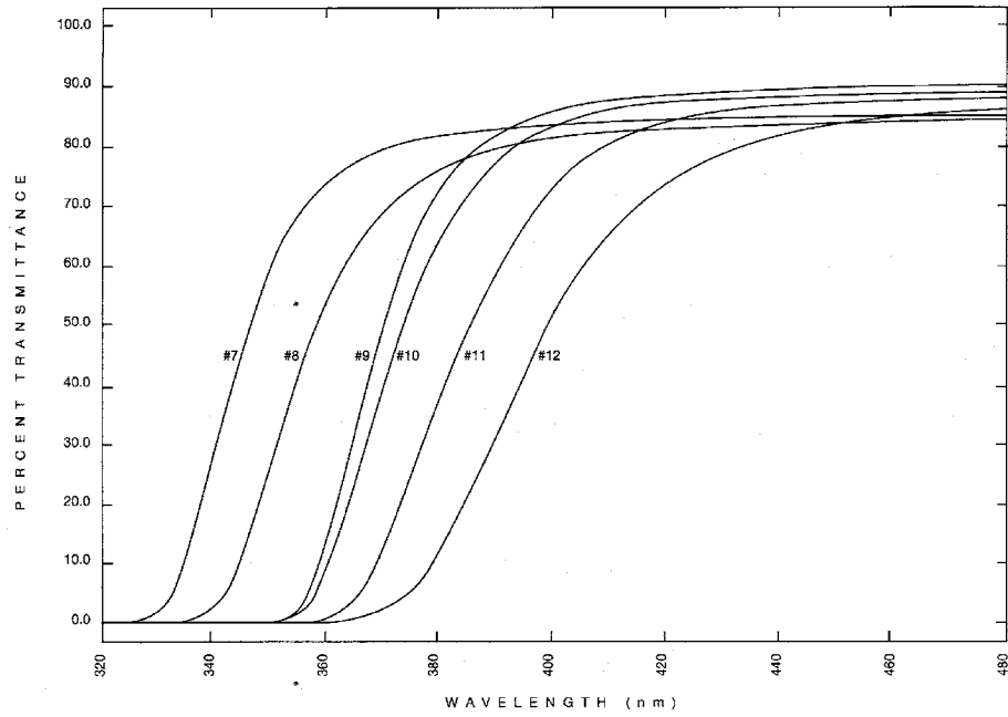
FIG. X1.2 Transmittance Curves of Sharp Cut-On UV/VIS Transmitting Filters 7 through 12 of a Typical Set
