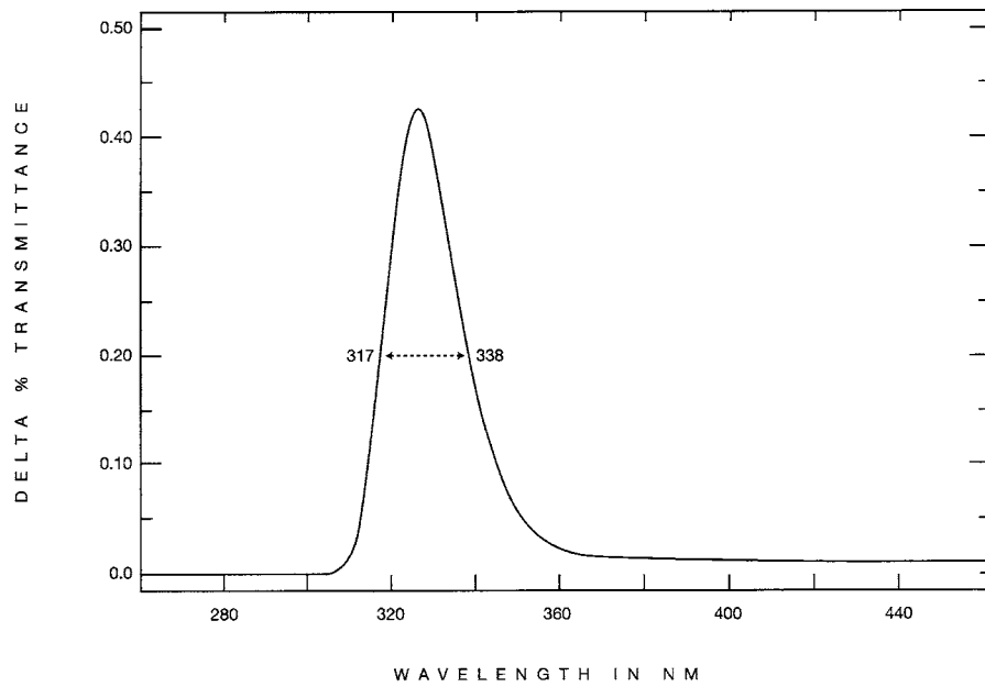
FIG. X1.3 Delta % Transmittance (Incremental UV) of Filters 5 minus 6 Shown in Fig. X1.1
