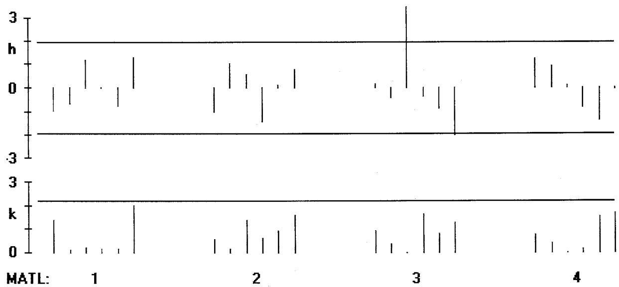
FIG. X1.3 Consistency Statistics by Material Analysis: \text{Log}_{10}(1/R_p) + 1
