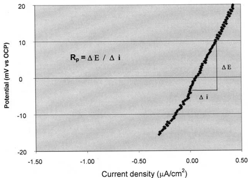
FIG. X1.4 Polarization Resistance Curve
