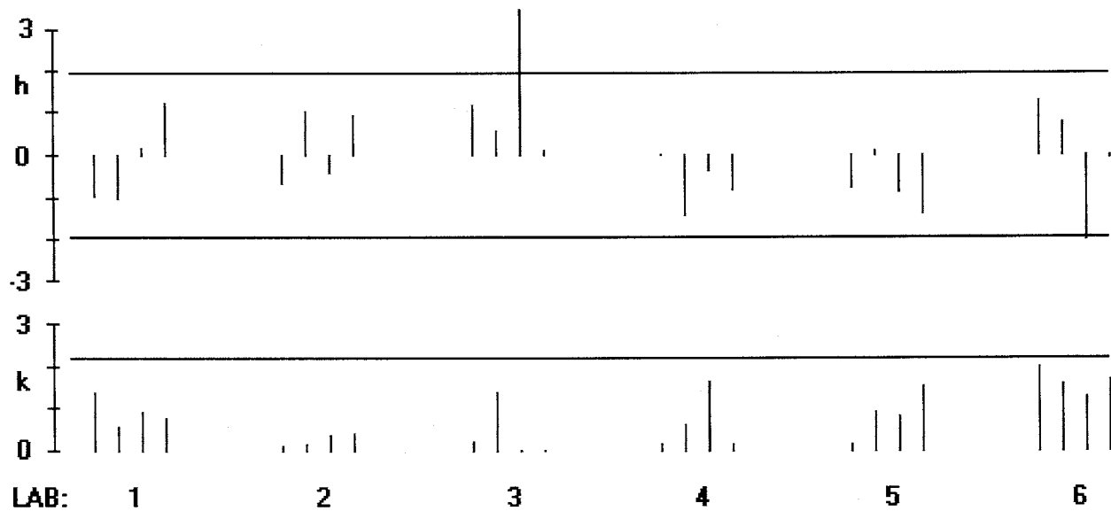
FIG. X1.2 Consistency Statistics by Laboratory Analysis: \text{Log}_{10}(1/R_p) + 1
