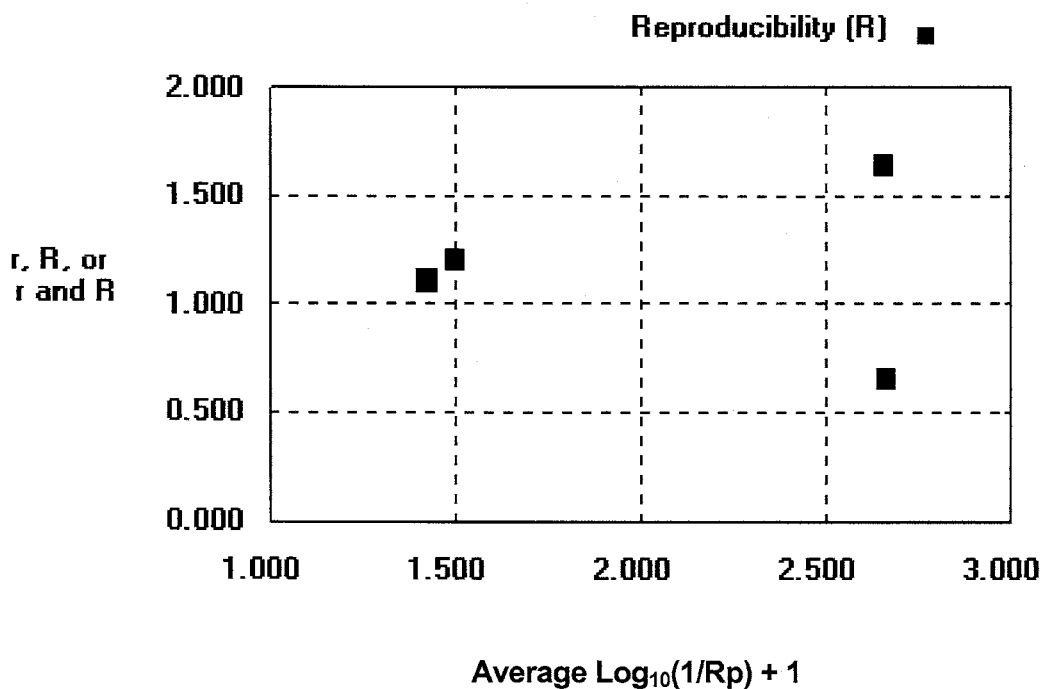
FIG. X1.1 r and R versus Material Averages Analysis: \text{Log}_{10}(1/R_p) + 1
