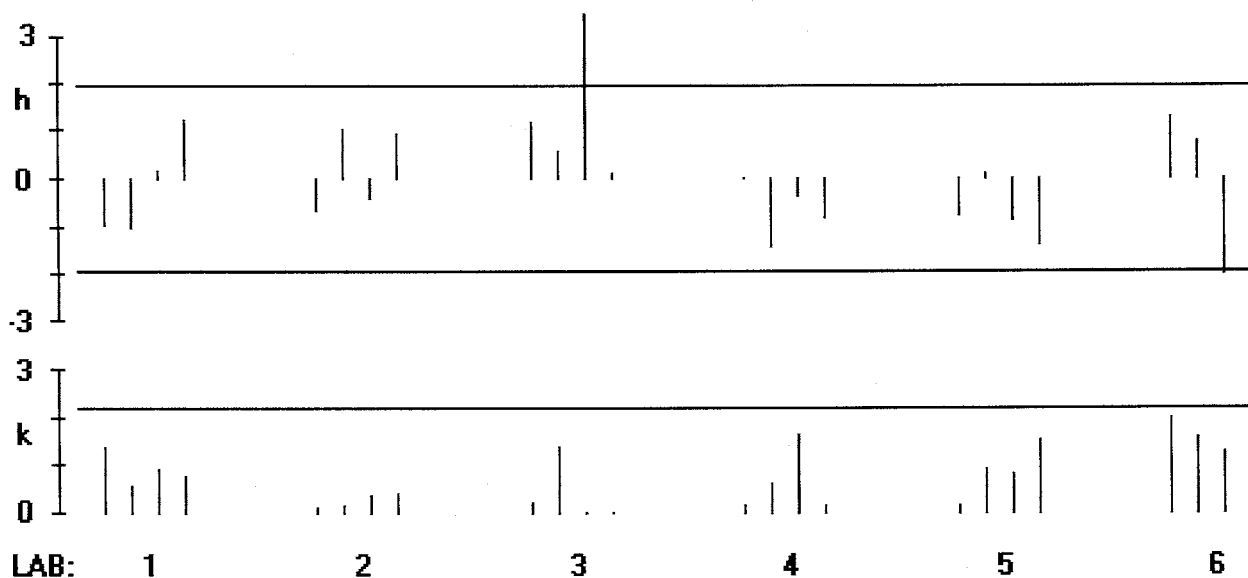
FIG. X1.2 Consistency Statistics by Laboratory Analysis: \log_{10}(1/R_p) + 1
