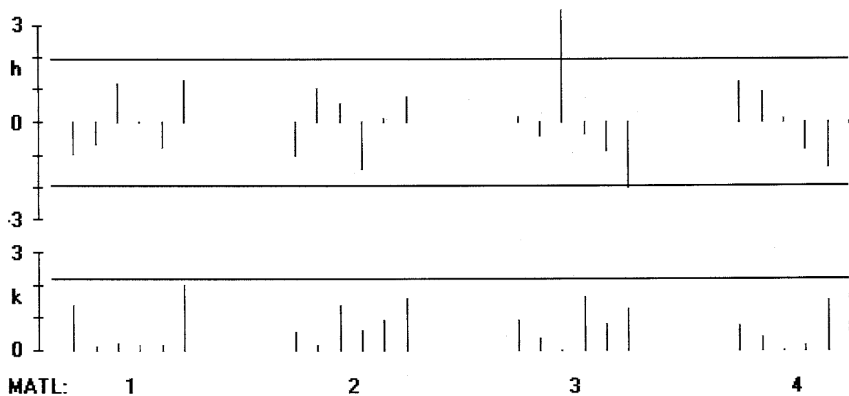
FIG. X1.3 Consistency Statistics by Material Analysis: \log_{10}(1/R_p) + 1
