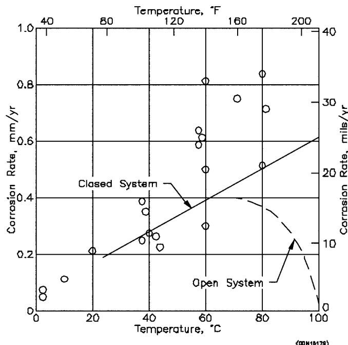
FIG. 1 Comparison of Actual Plant CUI Corrosion Rates Measurements (Open Data Points Shown is for Plant CUI) with Laboratory Corrosion Data Obtained in Open and Closed Systems
