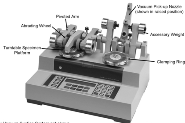
FIG. 1 Rotary Platform, Double-Head (RPDH) Abraser
