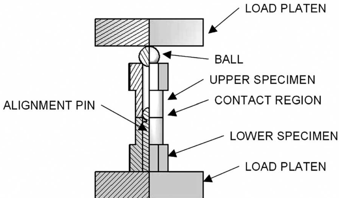
FIG. 3 Schematic Diagram of Galling Test Setup
