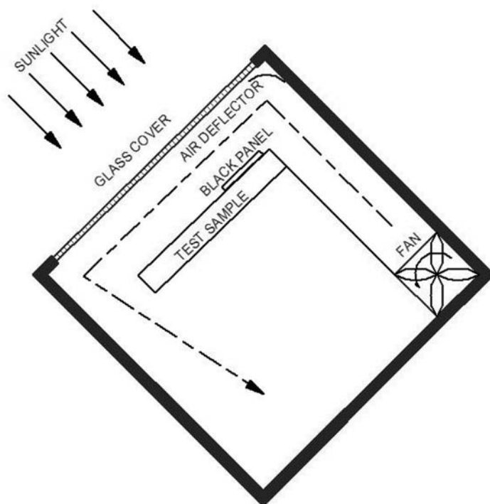
FIG. 1 Diagram of Typical Enclosure with Air Circulation
