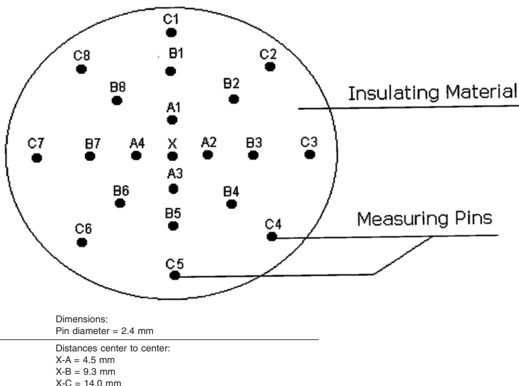
FIG. 7 Schematic Diagram Indicating the Positions of Measurement Pins in the Wettability Apparatus (Spreading Method)
