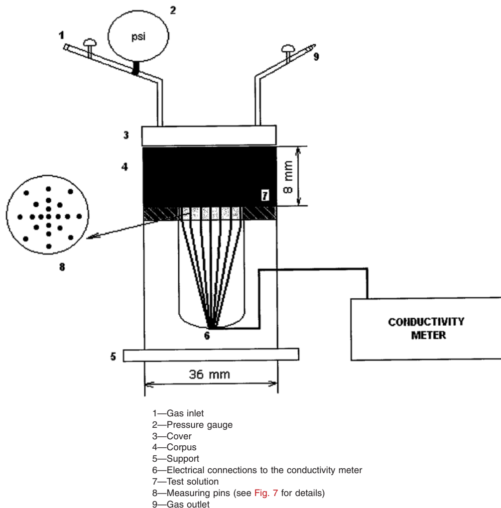
FIG. 6 Schematic Diagram of an Apparatus to Determine Wettability by Spreading
