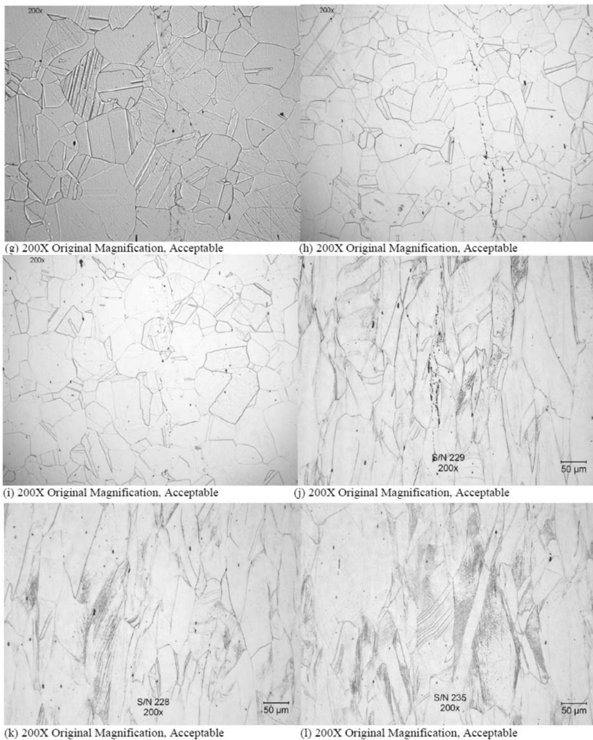
FIG. 2 Acceptable Microstructures Exhibiting the Absence of Significant mu Phase (continued)
