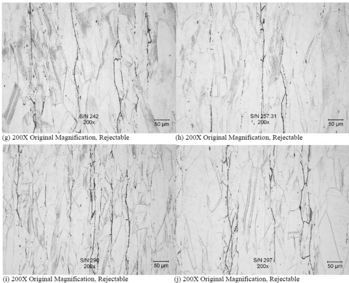
FIG. 3 Rejectable Microstructures Exhibiting the Presence of Significant \mu Phase (continued)
