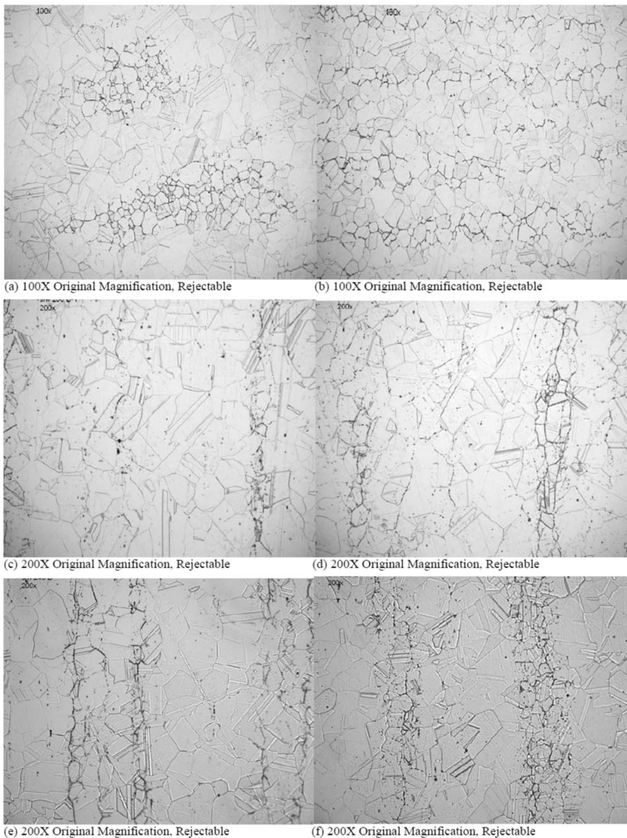
FIG. 3 Rejectable Microstructures Exhibiting the Presence of Significant mu Phase
