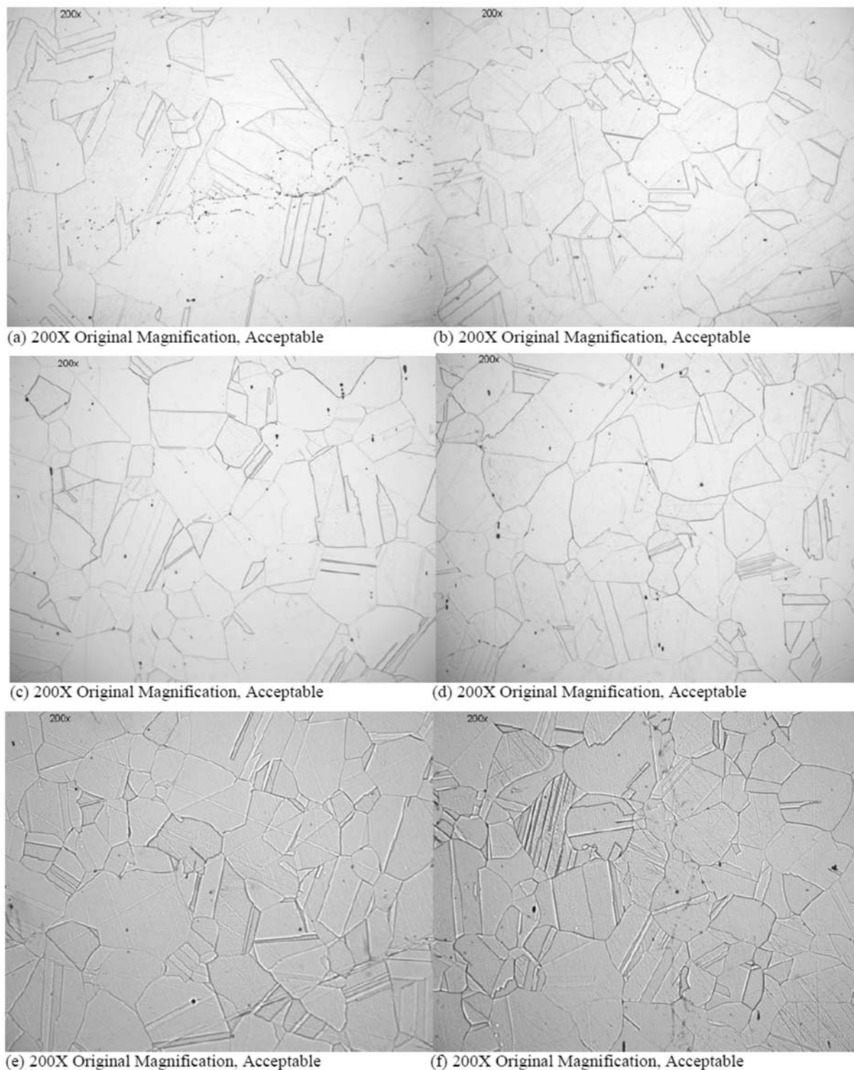
FIG. 2 Acceptable Microstructures Exhibiting the Absence of Significant mu Phase
