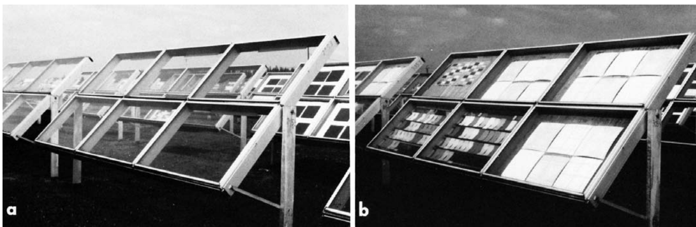
FIG. 1 a and 1b Typical Passively-Ventilated Under Glass Exposure Cabinet, Type A
