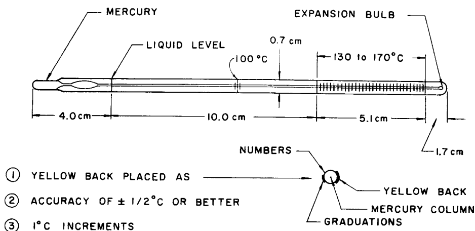
FIG. X1.5 Design of Thermometer for Use in Flask of Fig. X1.2
