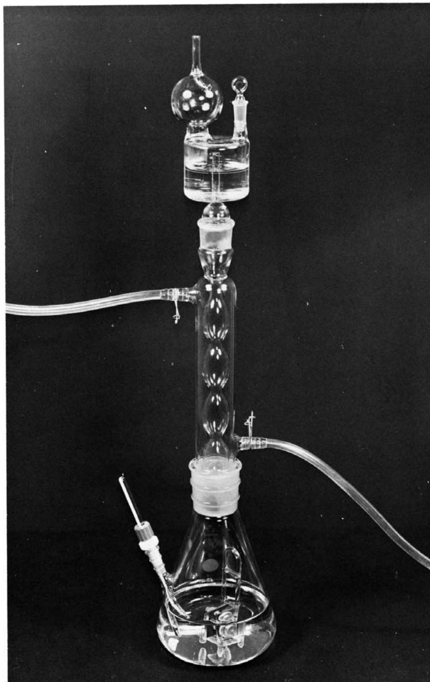
FIG. X1.1 Assembly of Glass Apparatus for Stress-Corrosion Test in Boiling Magnesium Chloride with U-Bend Specimen in Place
