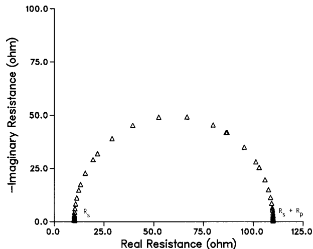
FIG. 8 Nyquist Plot for Equivalent Circuit of Fig. 7
