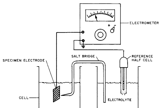
NOTE—The electrode potential of specimen is negative as shown. FIG. 1 Schematic Diagram of an Apparatus to Measure Electrode Potential of a Specimen
