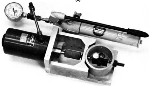
FIG. 3 Sustained Load Devices Using Ring Frames (8)
